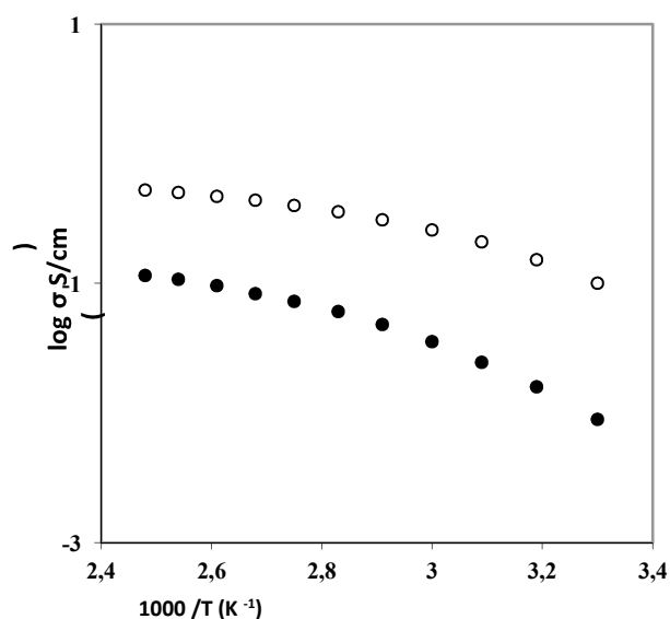
Figure 4. Variation of log conductivity with reciprocal temperature for nanocomposite plasticized polymer electrolytes containing PMMA+10wt% NH 4 CF 3 SO 3 +50wt% DEC (●) +5wt% SiO 2 and PMMA+10wt% NH 4 CF 3 SO 3 +50wt% DMA (○) + 3wt% SiO 2
