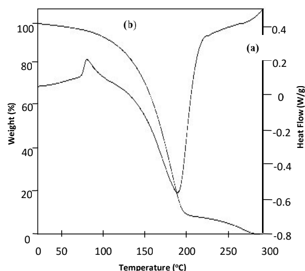
Figure 6. DSC (a) and TGA (b) plots for nanocomposite plasticized polymer electrolyte containing PMMA+ 10wt% \text{NH}_4\text{CF}_3\text{SO}_3 +50wt% DMA (○) + 5wt% \text{SiO}_2
