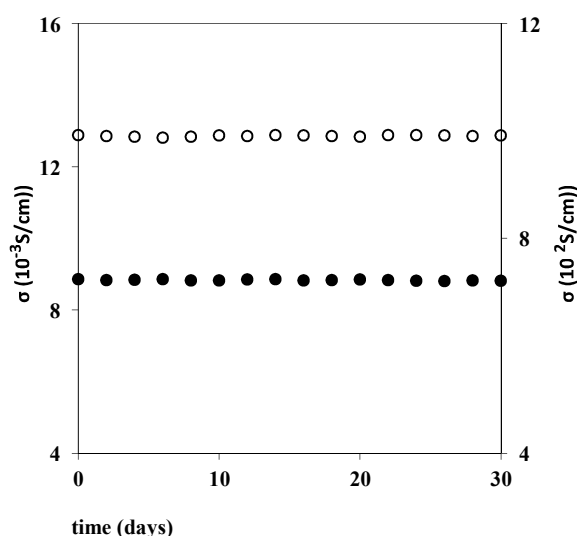
Figure 5. Variation of ionic conductivity with time for nanocomposite plasticized polymer electrolytes containing PMMA+10wt% \text{NH}_4\text{CF}_3\text{SO}_3 +50wt% DEC (●)+5wt% \text{SiO}_2 and PMMA+ 10wt% \text{NH}_4\text{CF}_3\text{SO}_3 +50wt% DMA (○) + 3wt% \text{SiO}_2
