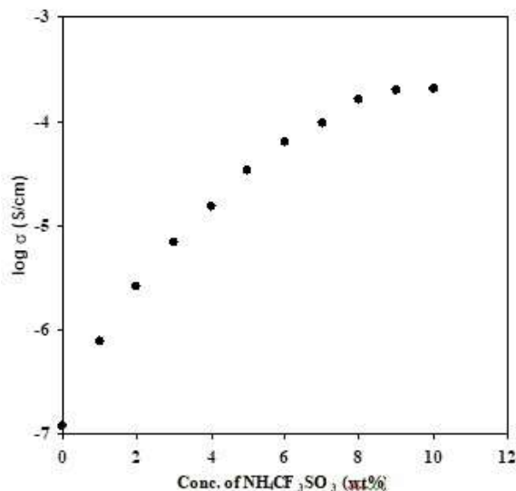
Figure 1. Variation of log conductivity ( \log \sigma ) for PMMA+ \text{NH}_4\text{CF}_3\text{SO}_3 polymer electrolytes with \text{NH}_4\text{CF}_3\text{SO}_3 concentration
